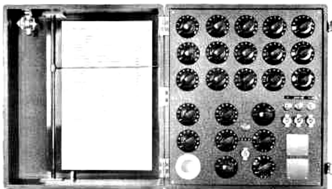
Fig. 18 RADIONIC ANALYTICAL COMPUTER—MK. II
